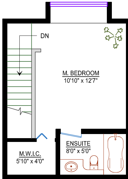
UPPER LEVEL 2 Area: 295 sq. ft.
