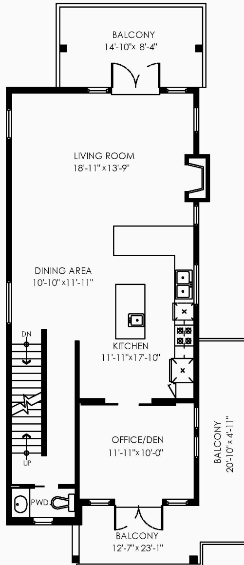
Main Floor Plan Floor Area: 876 sq.ft. Ceiling Height: 9 ft.
