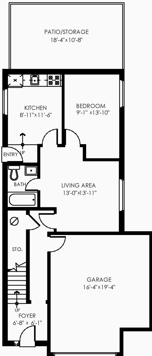
Lower Floor Plan Floor Area: 680 sq.ft. Ceiling Height: 8 ft.
